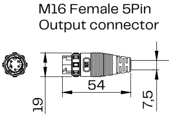
Connector SCALE 1:3
