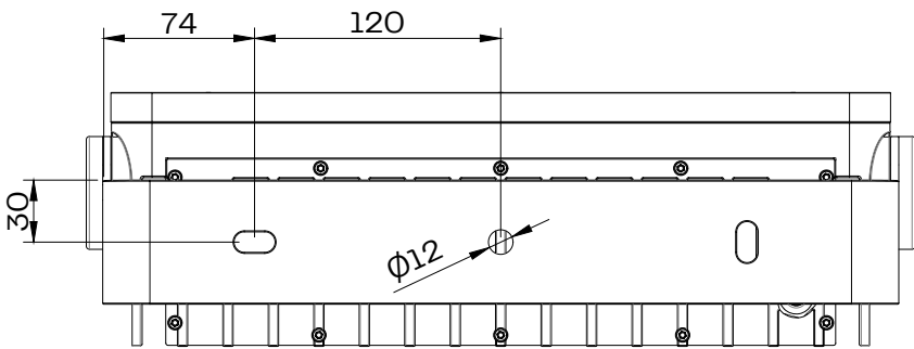
Mounting bracket SCALE 1:4
