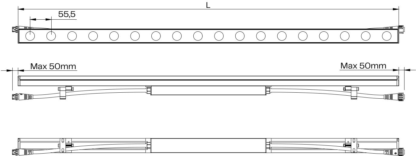
Fixture SCALE 1:6
