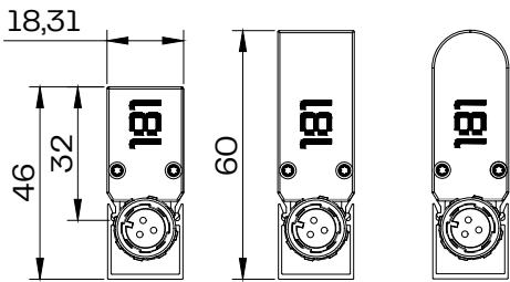
Side view SCALE 1:2
