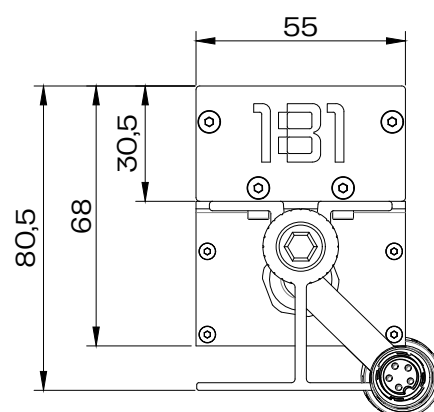
Side view SCALE 1:2
