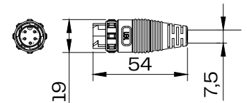
Connector SCALE 1:3
