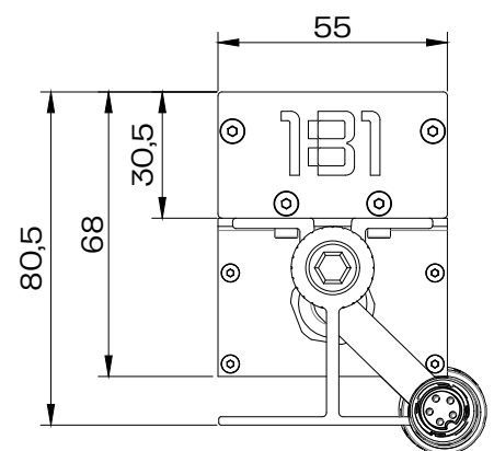
Side view SCALE 1:2
