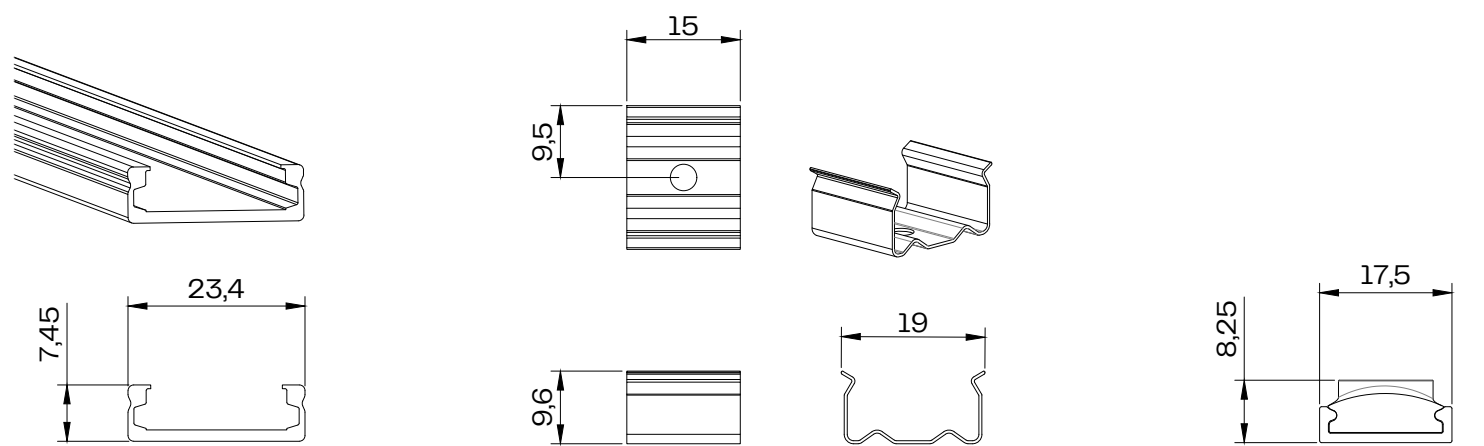
Mounting profile SCALE 1:1
