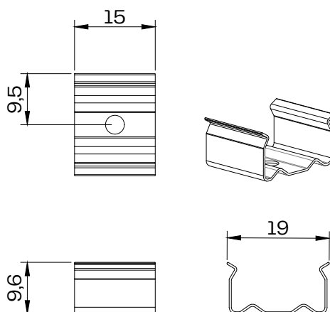
Mounting clip SCALE 1:1
