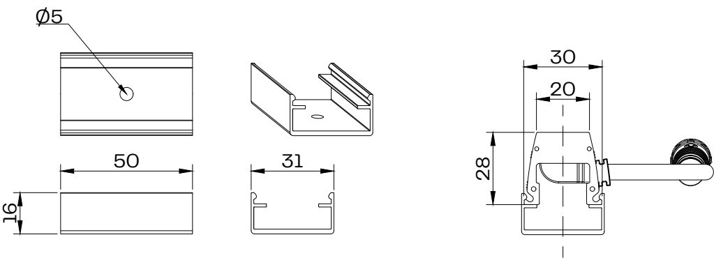
Mounting clip SCALE 1:2
