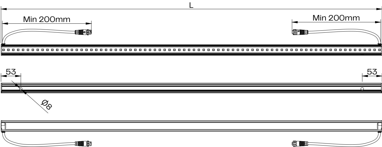
Fixture SCALE 1:6
