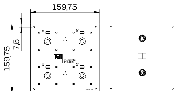
Panel 16P
