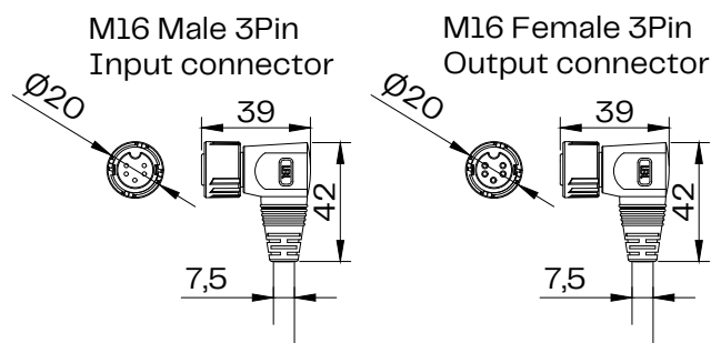
Connector
