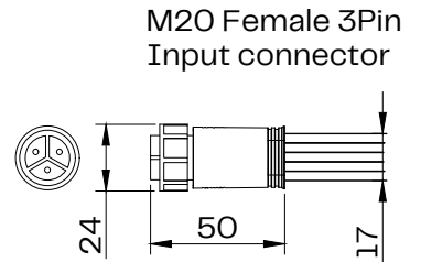
Connector SCALE 1:3
