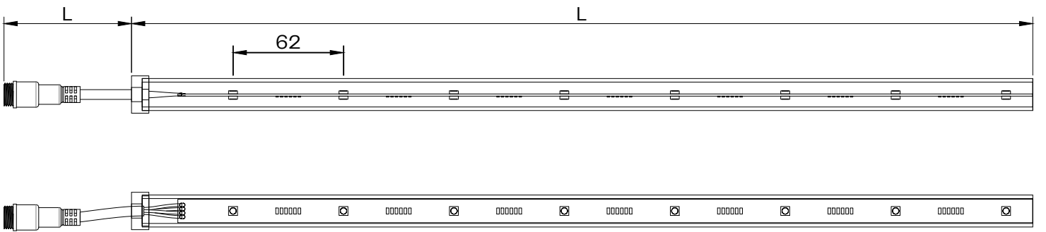
Fixture SCALE 1:3
