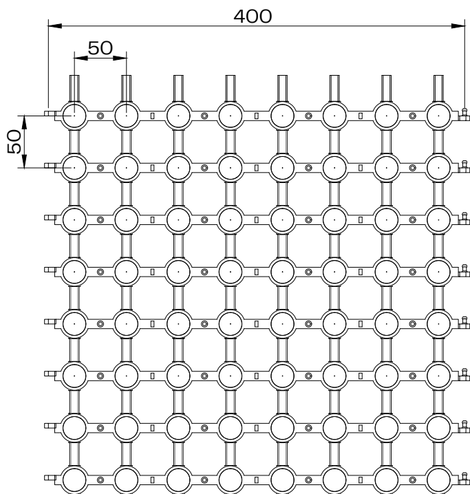
Front view SCALE 1:5
