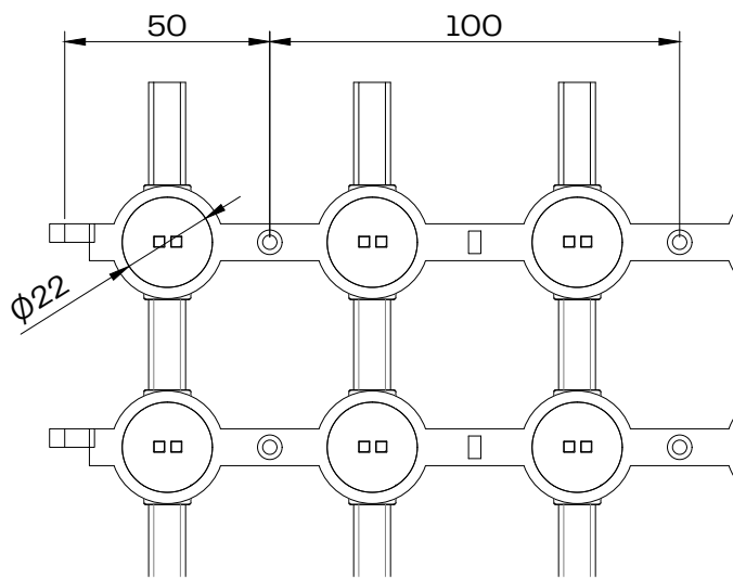
Front view SCALE 1:2
