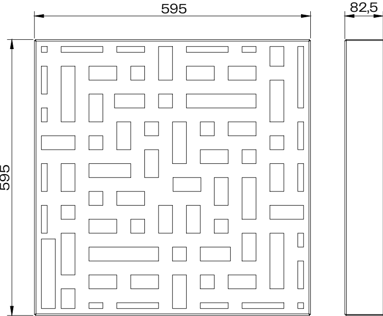
Maze SCALE 1:8
