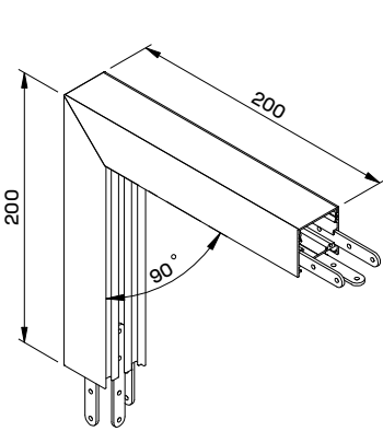
2-Way down Scale 1:5
