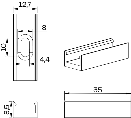
Mounting clip SCALE 1:1
