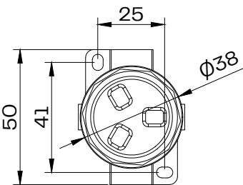
Top view SCALE 1:2
