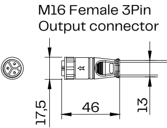
Connector SCALE 1:3
