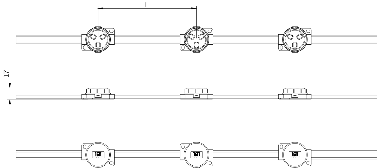
LED Module SCALE 1:3
