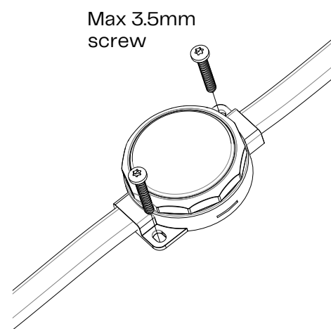
Screw fixation
