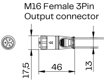
Connector SCALE 1:3
