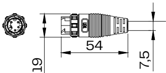
Connector SCALE 1:3
