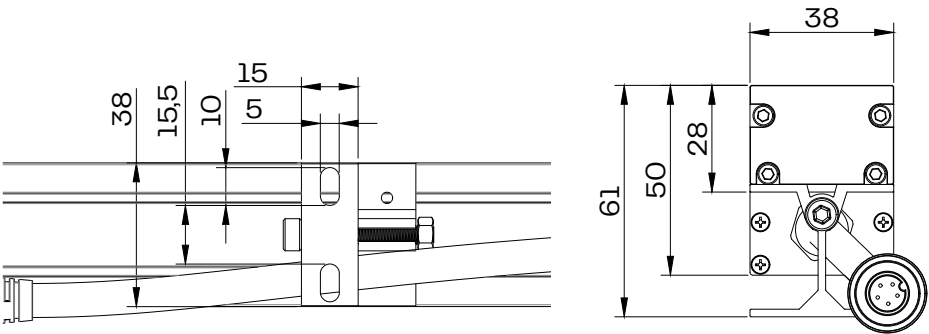
Mounting bracket SCALE 1:2
