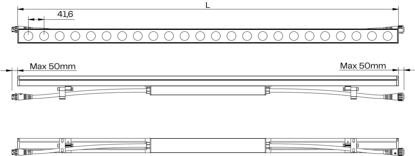
Fixture SCALE 1:6
