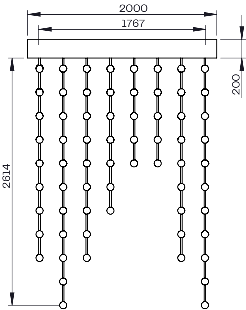
Side View SCALE 1:40
