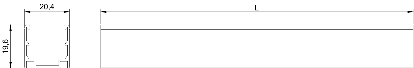
Neonflex Topview Mounting profile SCALE 1:1
