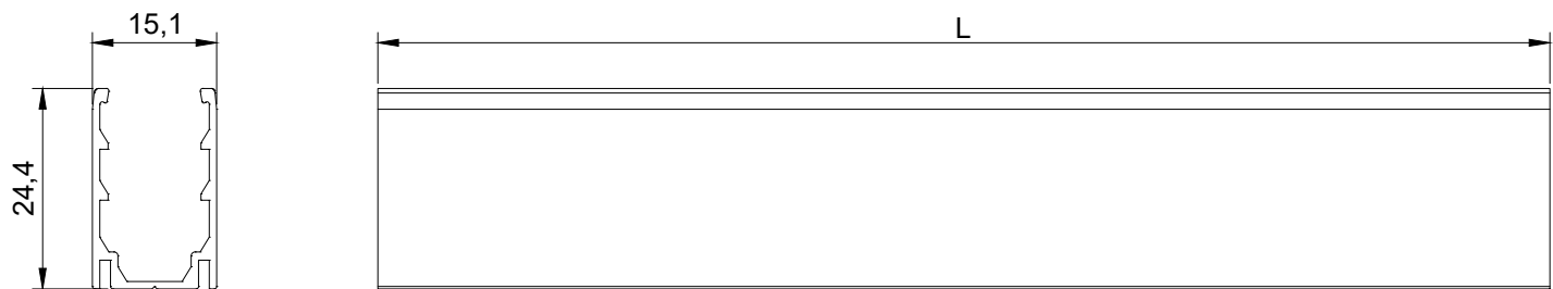
Neonflex Sideview Mounting profile SCALE 1:1
