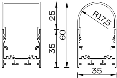
Cover high square and round SCALE 1:2
