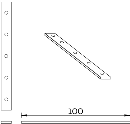
Extension module straight SCALE 1:2
