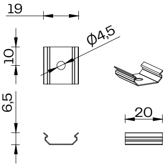
Mounting clip SCALE 1:2
