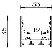
Side view SCALE 1:2
