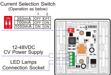
Terminal Description
